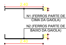
ARMADURA DA BASE: N1: 22 Ø3/8" x 2.60m N2: 22 Ø3/8" x 2.90m
